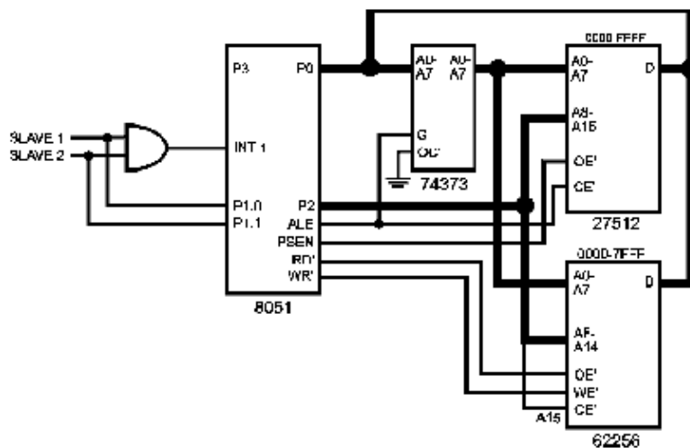
图0-1 INT1被共用
