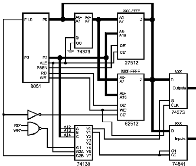
图0-3 RAM和I/O重叠
