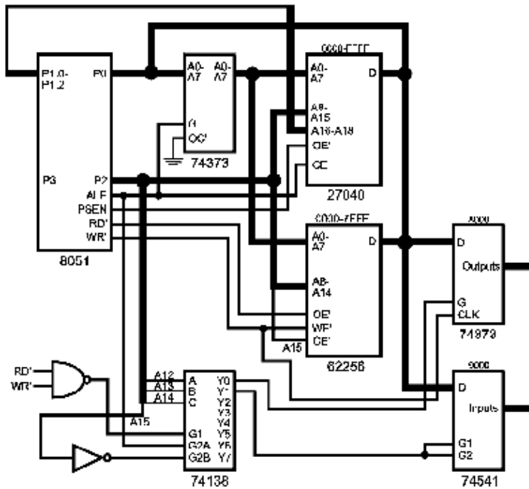
图0-5 页寻址EPROM
