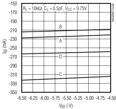
SUPPLY CURRENT, I EE vs. V EE
