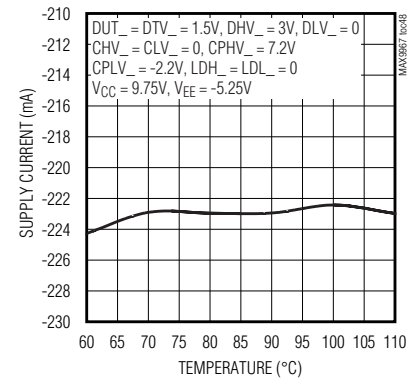
I EE vs. TEMPERATURE
