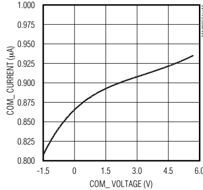
INPUT CURRENTS vs. INPUT VOLTAGE, COM_
