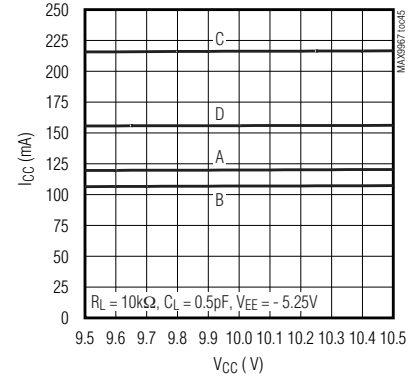
SUPPLY CURRENT, I CC vs. V CC
