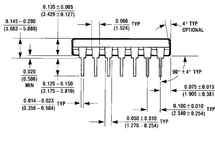
14-Lead Molded Dual-In-Line Package (N) Order Number DM74LS74AN NS Package Number N14A
