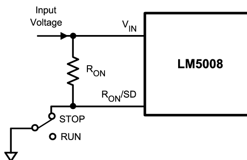
FIGURE 11. Shutdown Implementation
