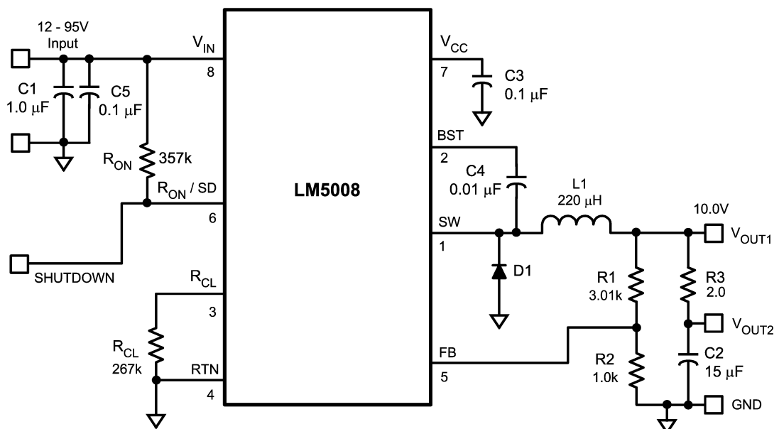
FIGURE 13. LM5008 Example Circuit
