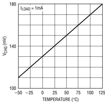
CHRG Pin Output Low Voltage vs Temperature
