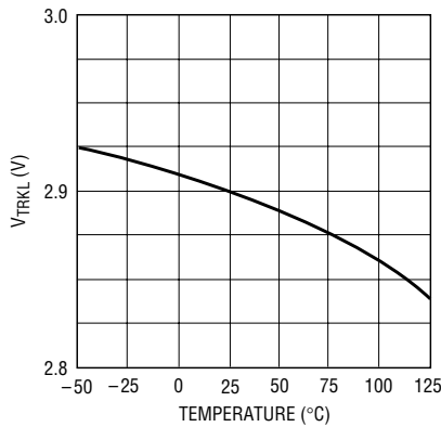
Trickle Charge Voltage vs Temperature
