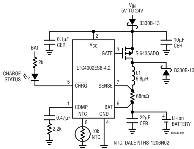
Figure 1. 1.5A Single Cell Li-Ion Battery Charger
