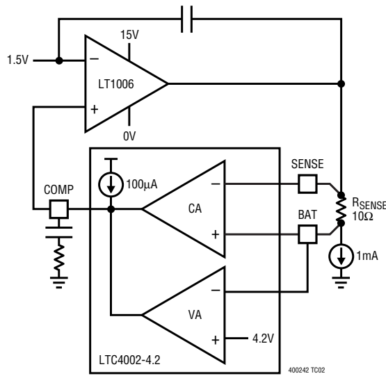
Test Circuit 2
