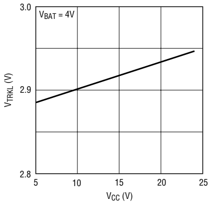
Trickle Charge Voltage vs V_{CC}
