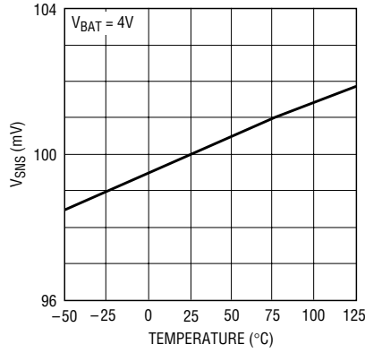
Current Mode Sense Voltage vs Temperature
