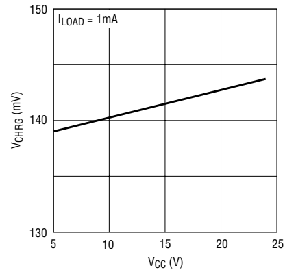
CHRG Pin Output Low Voltage vs V_{CC}
