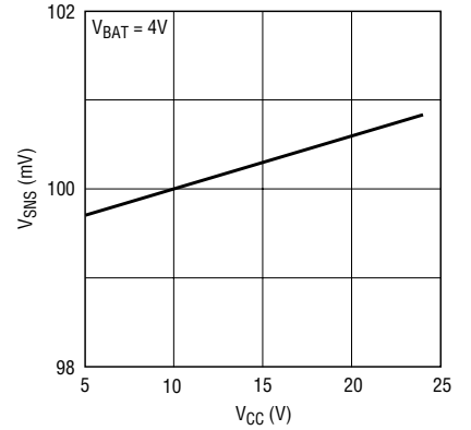
Current Mode Sense Voltage vs V_{CC}
