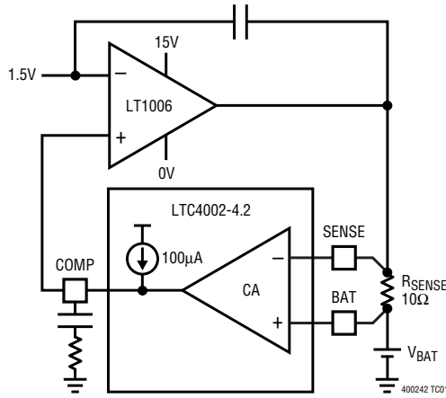
Test Circuit 1
