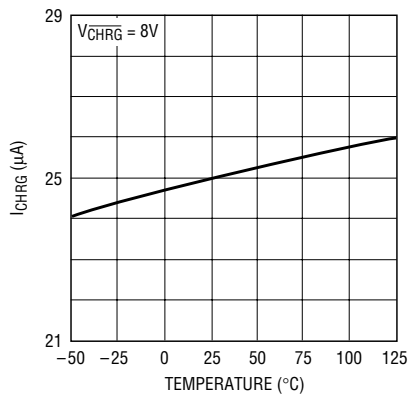
CHRG Pin Weak Pull-Down Current vs Temperature
