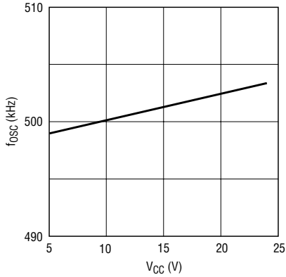
Oscillator Frequency vs V_{CC}
