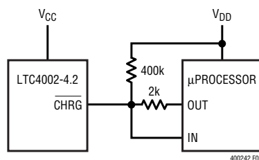
Figure 2. Microprocessor Interface
