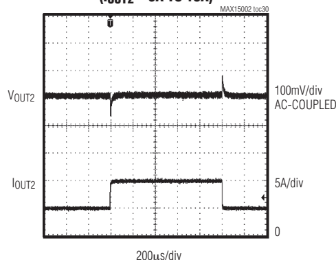
LOAD-TRANSIENT RESPONSE ( I_{OUT2} = 5A TO 10A )
