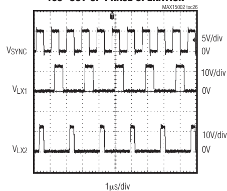
180° OUT-OF-PHASE OPERATION
