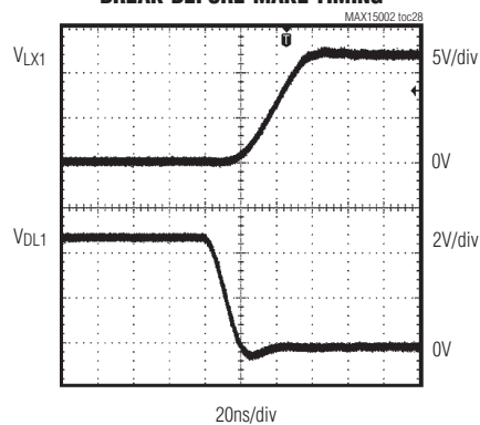
BREAK-BEFORE-MAKE TIMING
