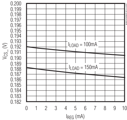
CS_ VOLTAGE vs. REG OUTPUT CURRENT
