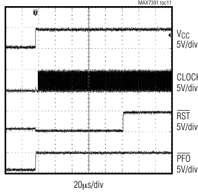
POWER-ON RESET BEHAVIOR
