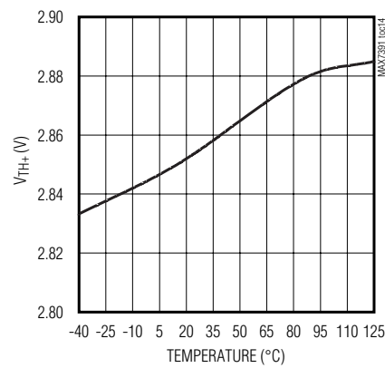
RIISING THRESHOLD vs. TEMPERATURE
