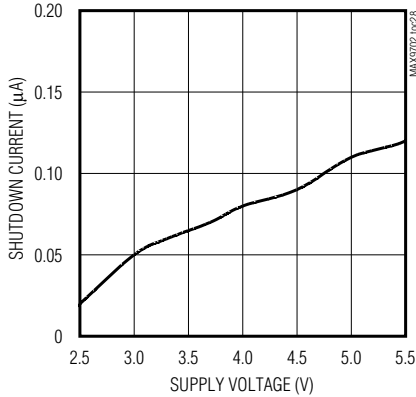
SHUTDOWN CURRENT vs. SUPPLY VOLTAGE (SPEAKER MODE)
