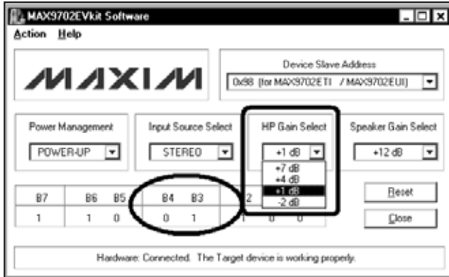
图5. HP Gain Select组合框
