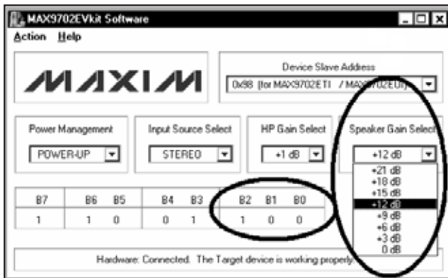
图6. Speaker Gain Select组合框
