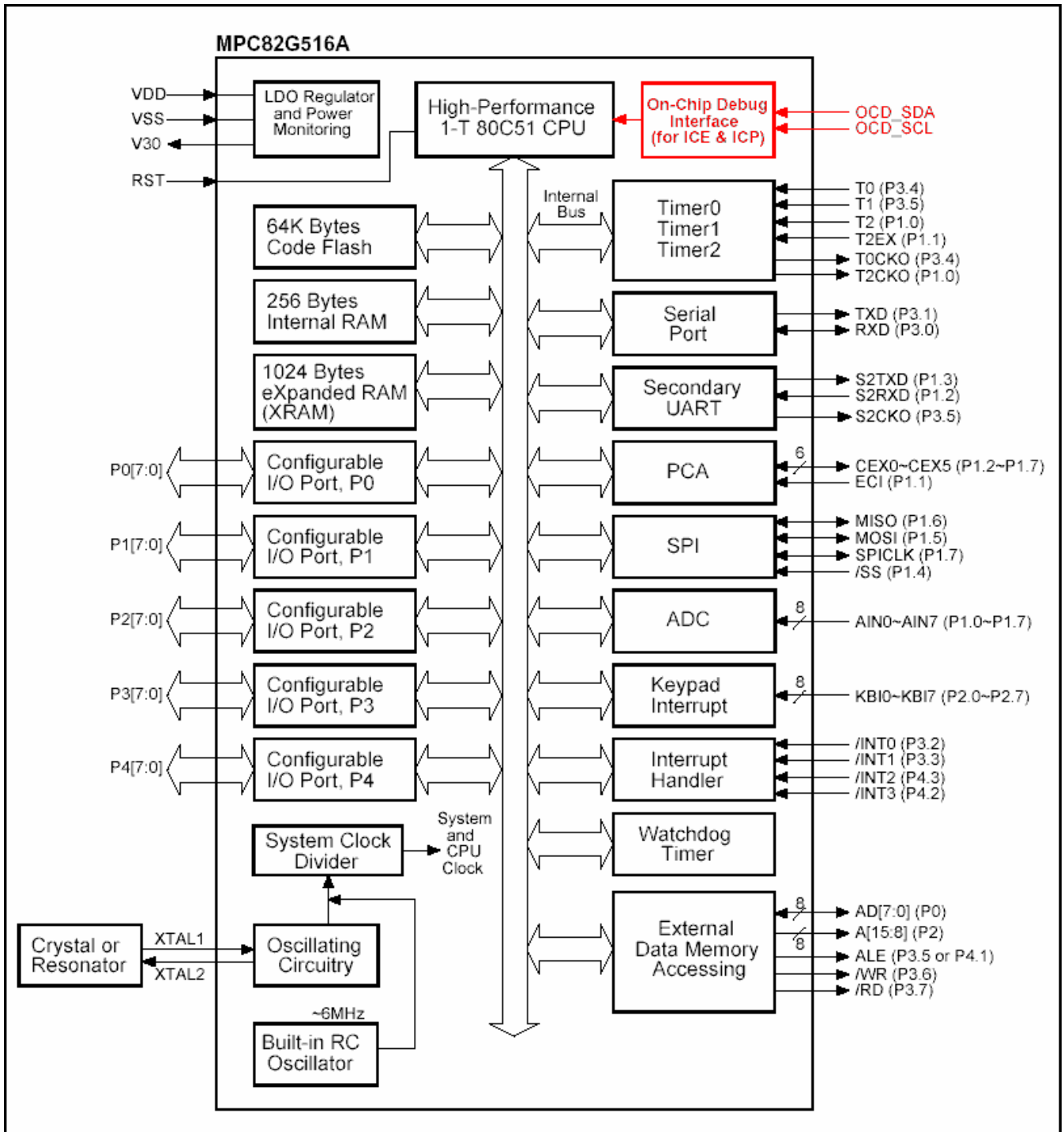
Figure 3-1. 方框图
