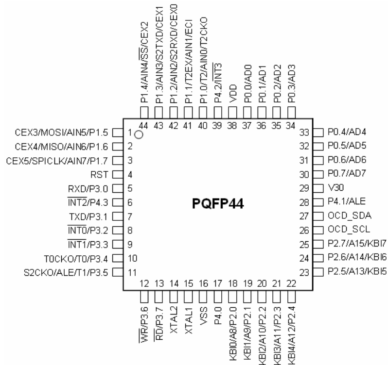
Figure 4-4. 引脚结构: 44-Pin PQFP
