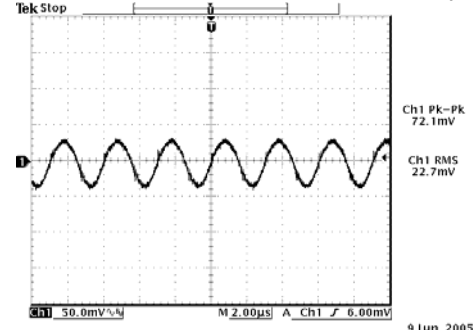
Ripple and noise at full load, 5.0 V/30 A output
