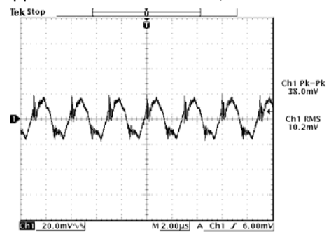
Ripple and noise at full load, 2.5 V/45 A output
