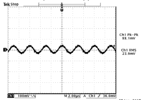
Ripple and noise at full load, 12 V/12 A output
