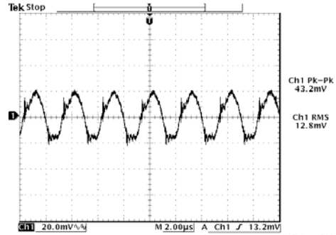
Ripple and noise at full load, 1.5 V/50 A output
