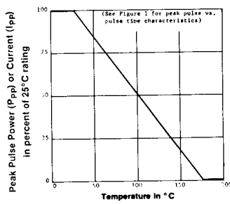
FIGURE 4 DERATING CURVE
