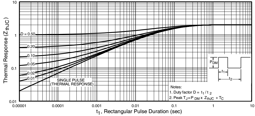
Fig. 4 - Max. Thermal Impedance Z_{thJC} Characteristics (Per Leg)
