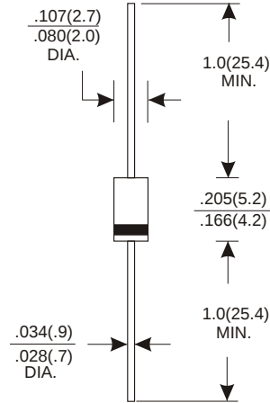
DO-41
