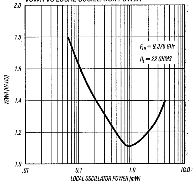
VSWR VS LOCAL OSCILLATOR POWER
