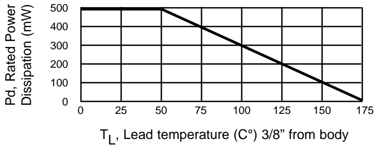
POWER DERATING CURVE
