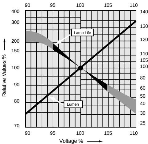
Life/Lumen-Volt Characteristic
