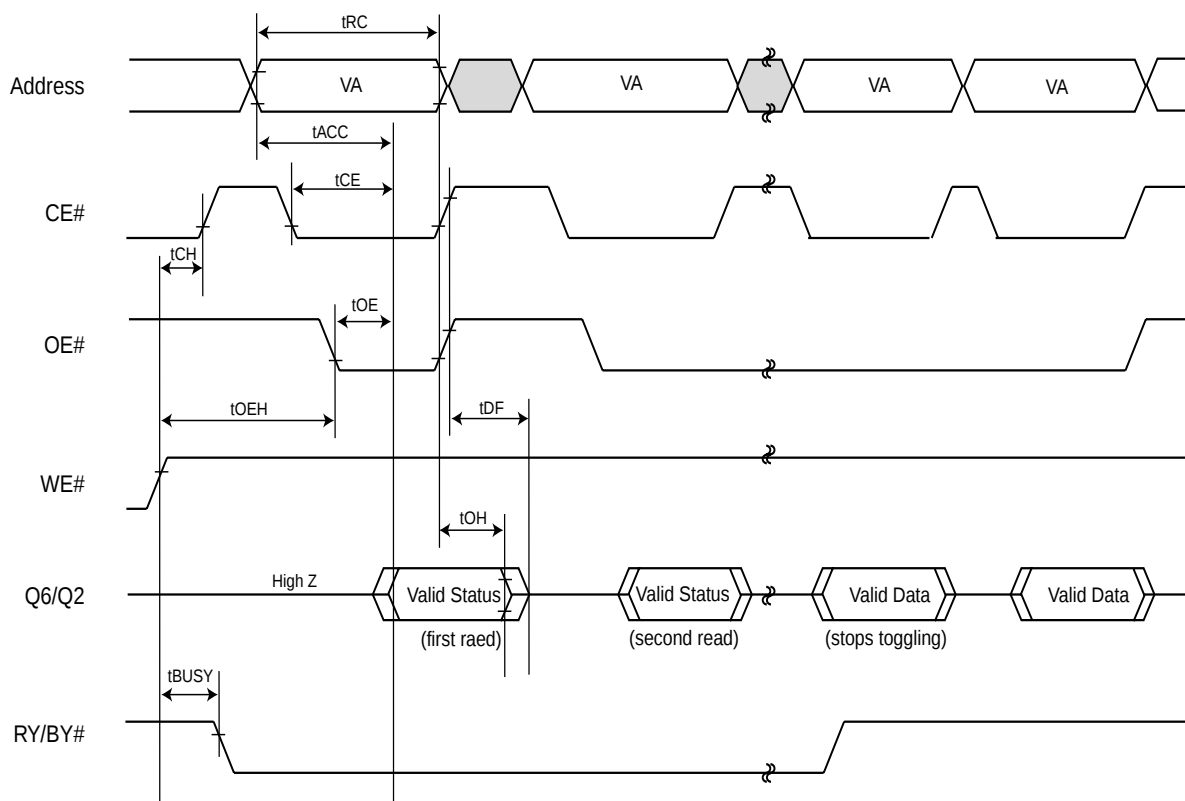
Figure 23. TOGGLE BIT TIMING WAVEFORMS (DURING AUTOMATIC ALGORITHMS)
