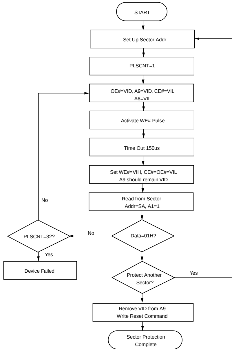
Figure 16. SECTOR PROTECTION ALGORITHM (A9, OE# Control)
