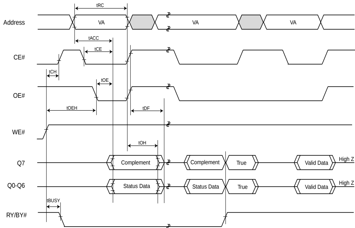
Figure 22. DATA# POLLING TIMINGS (DURING AUTOMATIC ALGORITHMS)
