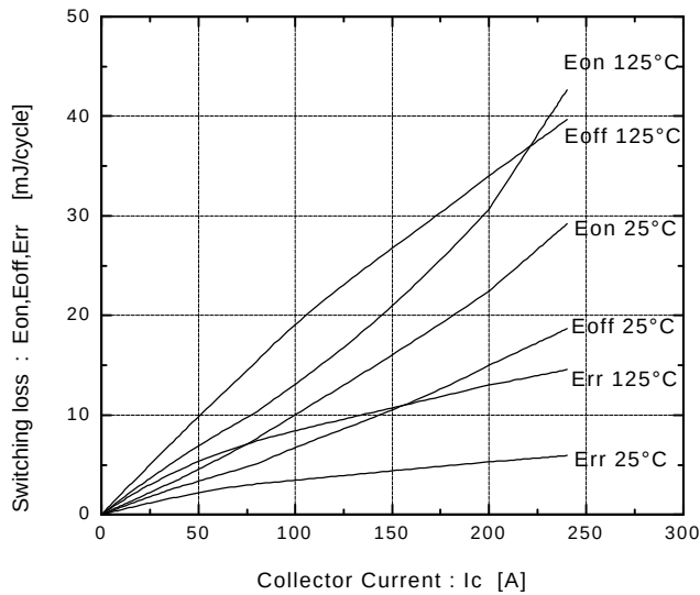
Switching loss vs. Collector current V_{CC}=600V , R_G=5.6\Omega , V_{GE}=\pm 15V
