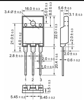
TO-3PML
