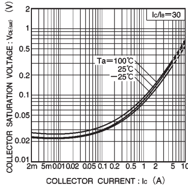
Fig.8 Collector-emitter saturation voltage vs. collector current (Ⅲ)
