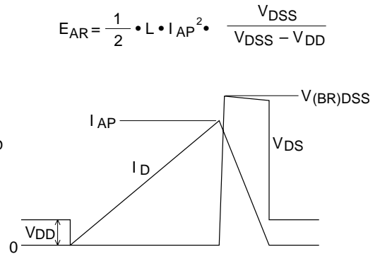
Avalanche Waveform
