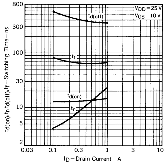
SWITCHING CHARACTERISTICS
