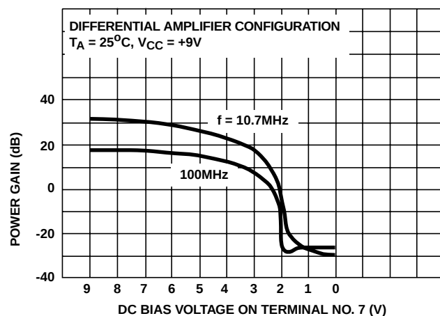
FIGURE 29. AGC CHARACTERISTICS
