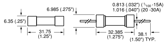
326 000 Series
