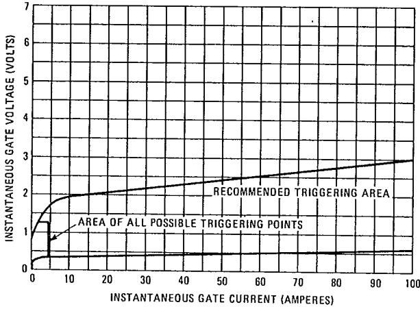
Fig. 9 - Gate Characteristics
