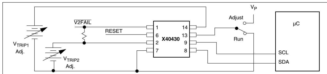
Figure 5. Sample V_{TBIP} Reset Circuit
