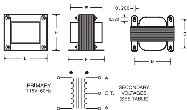
Dimensions, Inches
