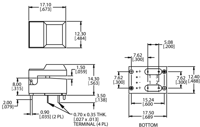
P.C. MOUNTING
