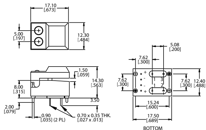
P.C. MOUNTING
