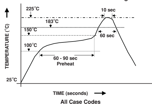
Recommended SnPb Reflow Soldering Profile
