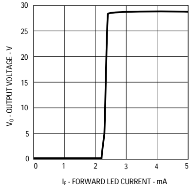
Figure 15. Transfer Characteristics
