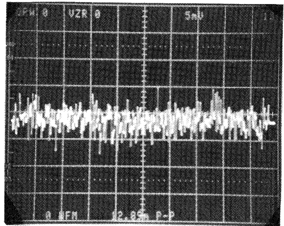
A_V = 25,000 , V_S = \pm 15V (12.89mV P,P RTO or 0.52μV P,P RTI) PEAK-TO-PEAK TOTAL NOISE 0.1Hz TO 1MHz
