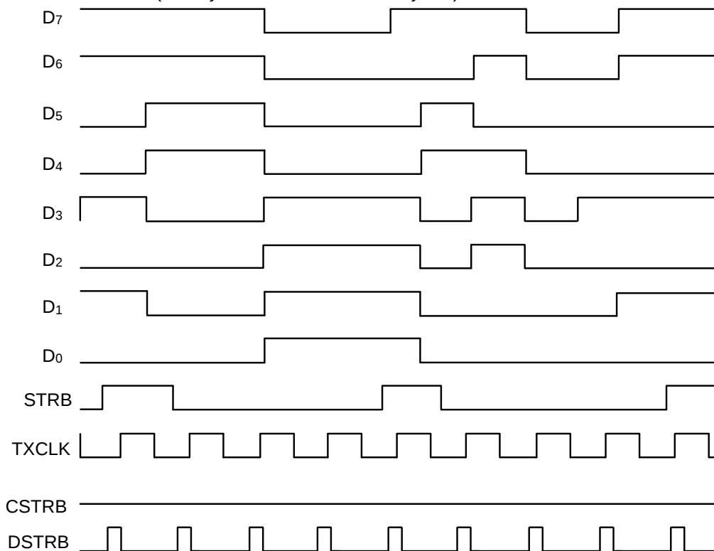
Figure 17 AUTORUN ACK 0 (No Sync Between Data Bytes)
