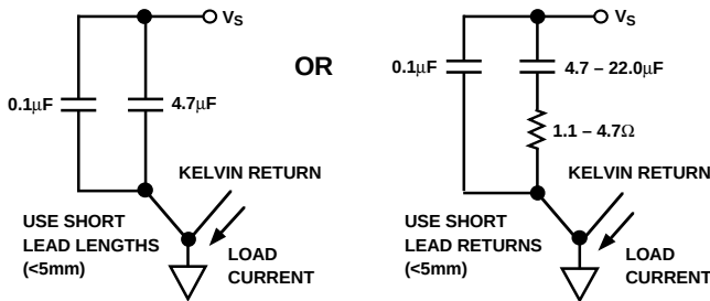
Figure 32. Recommended Power Supply Bypassing
