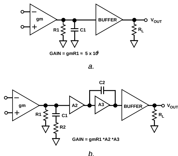
Figure 27. Model of AD797 vs. That of a Typical Three-Stage Amplifier
