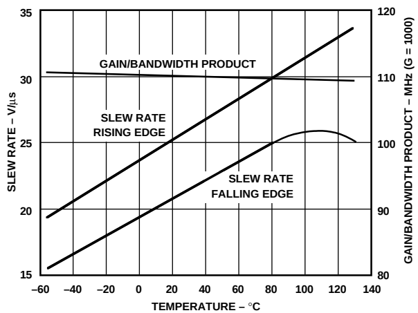
Figure 16. Slew Rate & Gain/Bandwidth Product vs. Temperature
