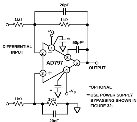
Figure 43. Differential Line Receiver
