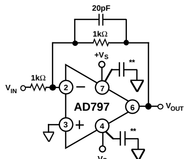
Figure 19. Inverter Connection
