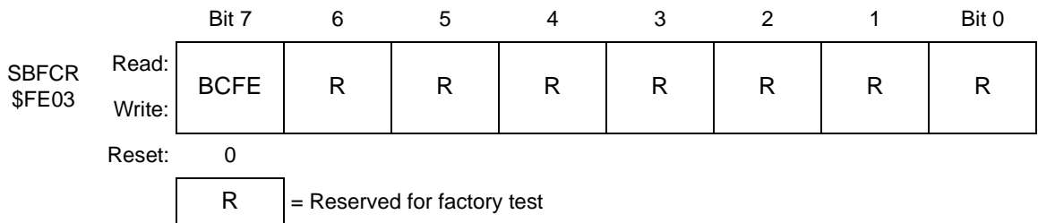
Figure 7-17. SIM Break Flag Control Register (SBFCR)
