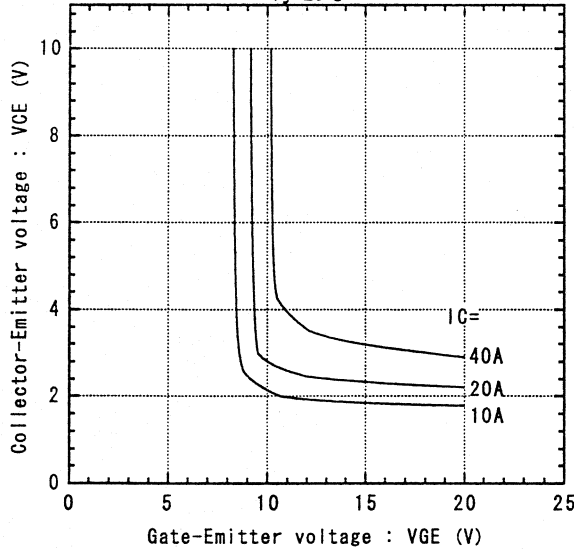
Collector-Emitter vs. Gate-Emmitter voltage T j =25°C
