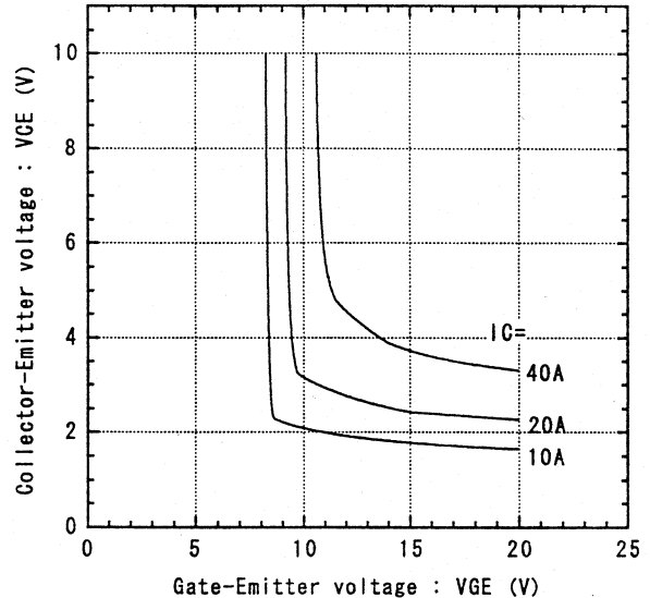
Collector-Emitter vs. Gate-Emmitter voltage T j =125°C
