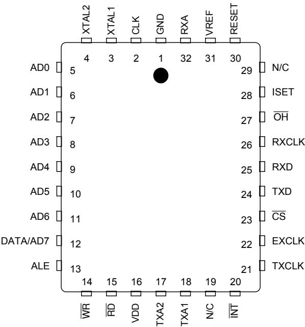
32-Lead PLCC 73K222BL-IH
