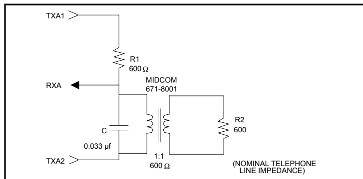
FIGURE 1: Analog Interface Hybrid Loading
