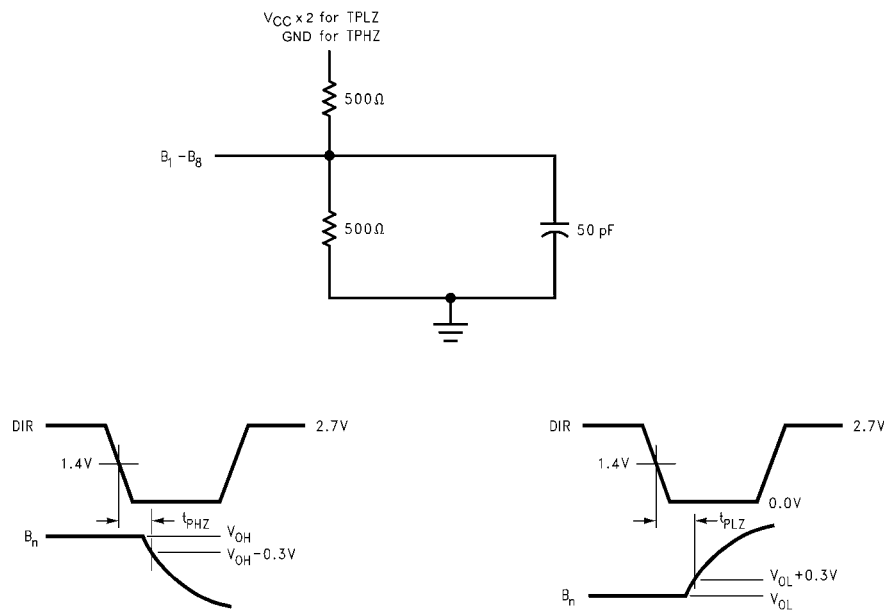
FIGURE 10. t PHZ and t PLZ Test Load and Waveforms DIR to B 1 -B 8
