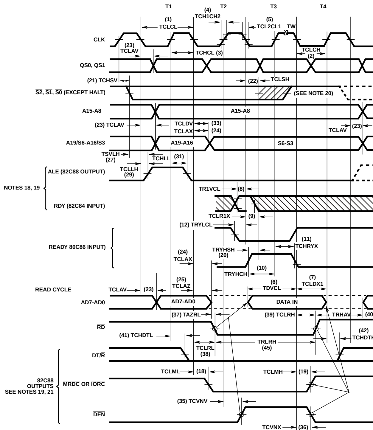
FIGURE 24. BUS TIMING - MAXIMUM MODE (USING 82C88)
