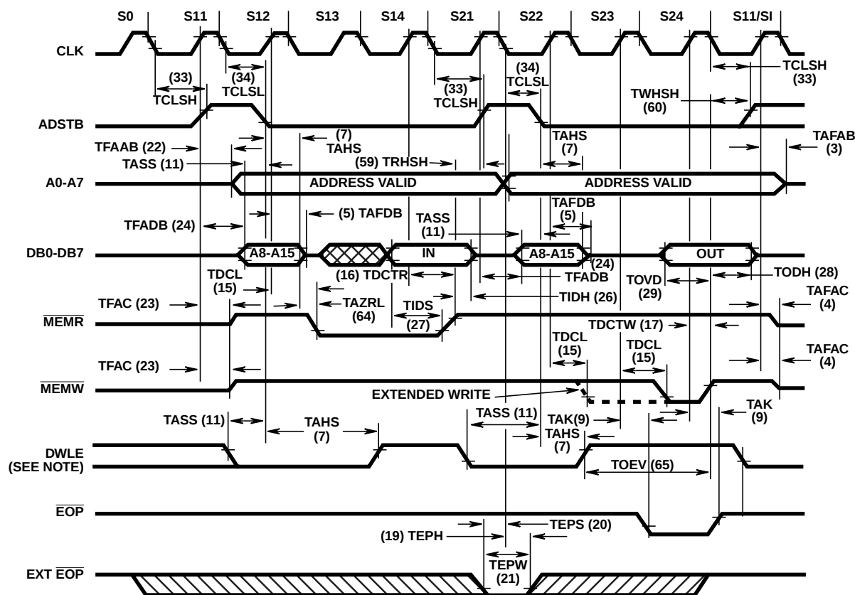
FIGURE 13. MEMORY-TO-MEMORY TRANSFER
