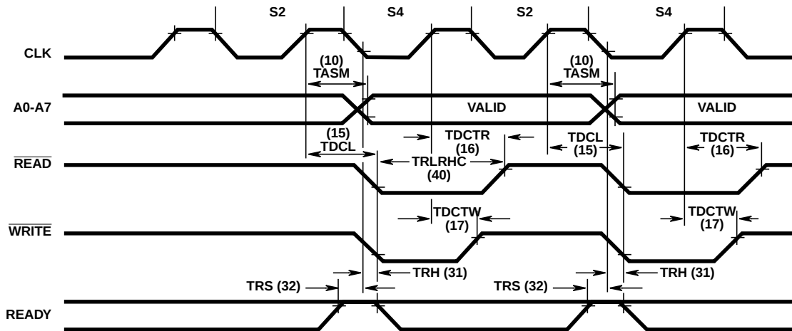
FIGURE 15. COMPRESSED TRANSFER
