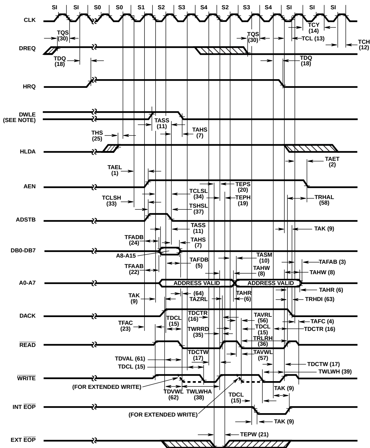
FIGURE 12. DMA TRANSFER
