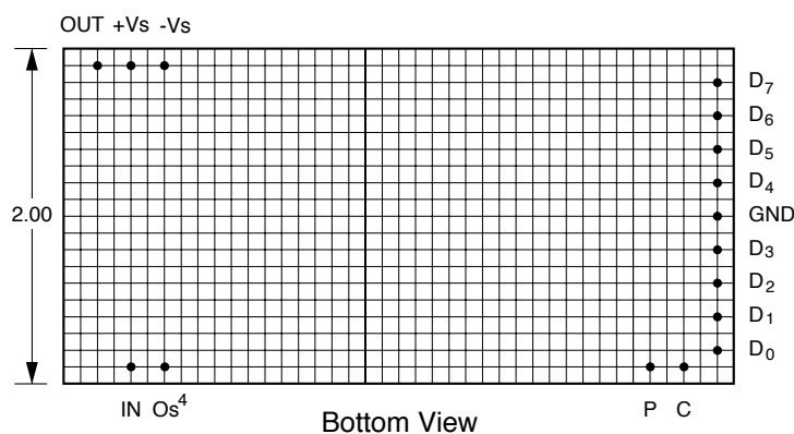
Filter Mounting Assembly-See FMA-03A
