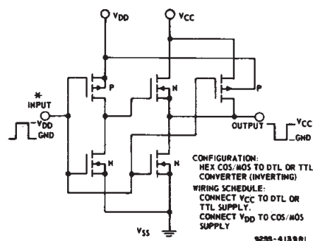
Fig. 1 – Schematic diagram of CD4009UB— 1 of 6 identical stages.
