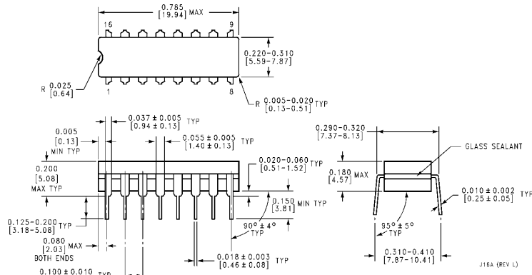
16-Lead Ceramic Dual-In-Line Package (J) Order Number 93L24DMQB NS Package Number J16A
