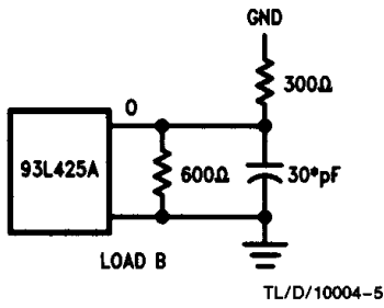
FIGURE 1. AC Test Output Load
