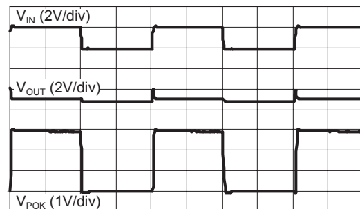
POK Output Response
