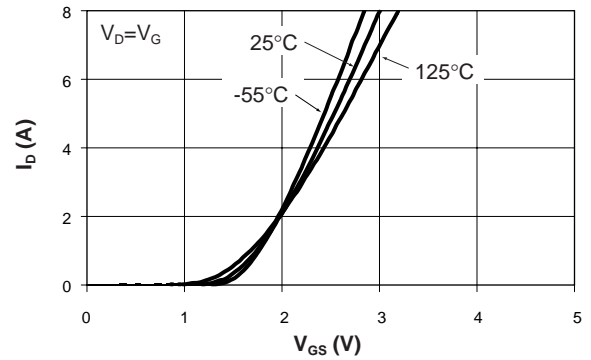
Transfer Characteristics
