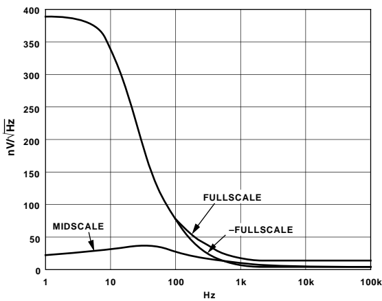
Figure 2. Noise Density
