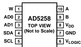
Figure 3. Pinout
