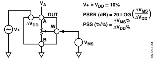
Figure 34. Test Circuit for Power Supply Sensitivity (PSS, PSSR)
