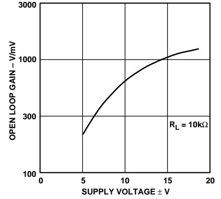
Figure 6. Open Loop Gain vs. Supply Voltage
