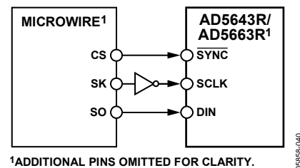
Figure 59. AD5623R/AD5643R/AD5663R to MICROWIRE Interface
