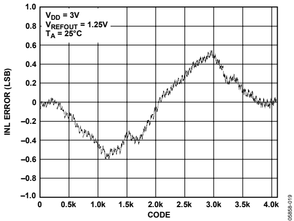
Figure 18. INL—AD5623R-3
