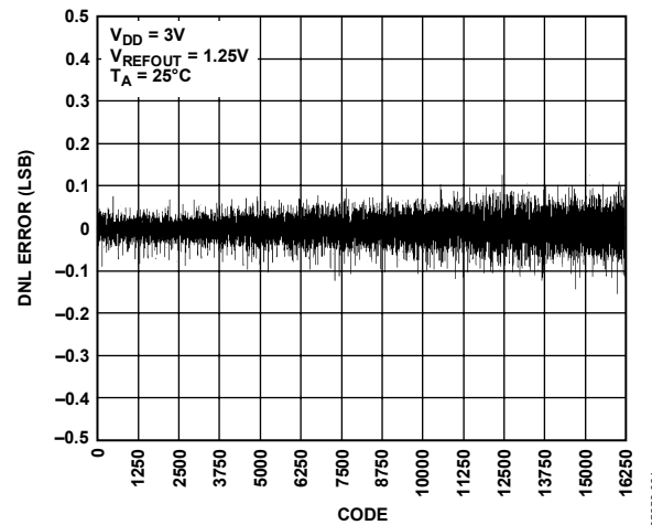
Figure 20. DNL—AD5643R-3
