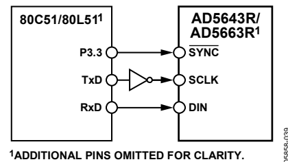
Figure 58. AD5623R/AD5643R/AD5663R to 80C51/80L51 Interface
