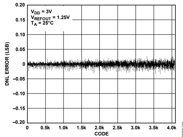
Figure 21. DNL—AD5623R-3
